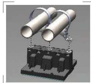
054: Two Elevated 1"-3" Pipe Rollers
