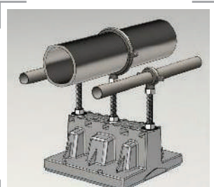
014: Elevated Split Ring Clamps
