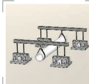
082: Two Blox Bridge with Underhung Piping
