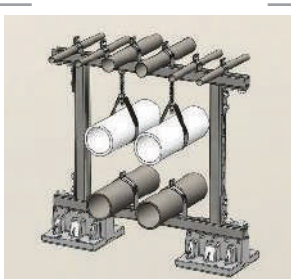
083: Two Blox 2-Tier Bridge Piping Rack
