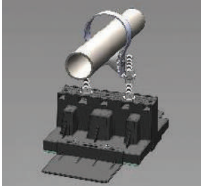
055: Blox with 1"-3" Pipe Roller & Securing Brackets
