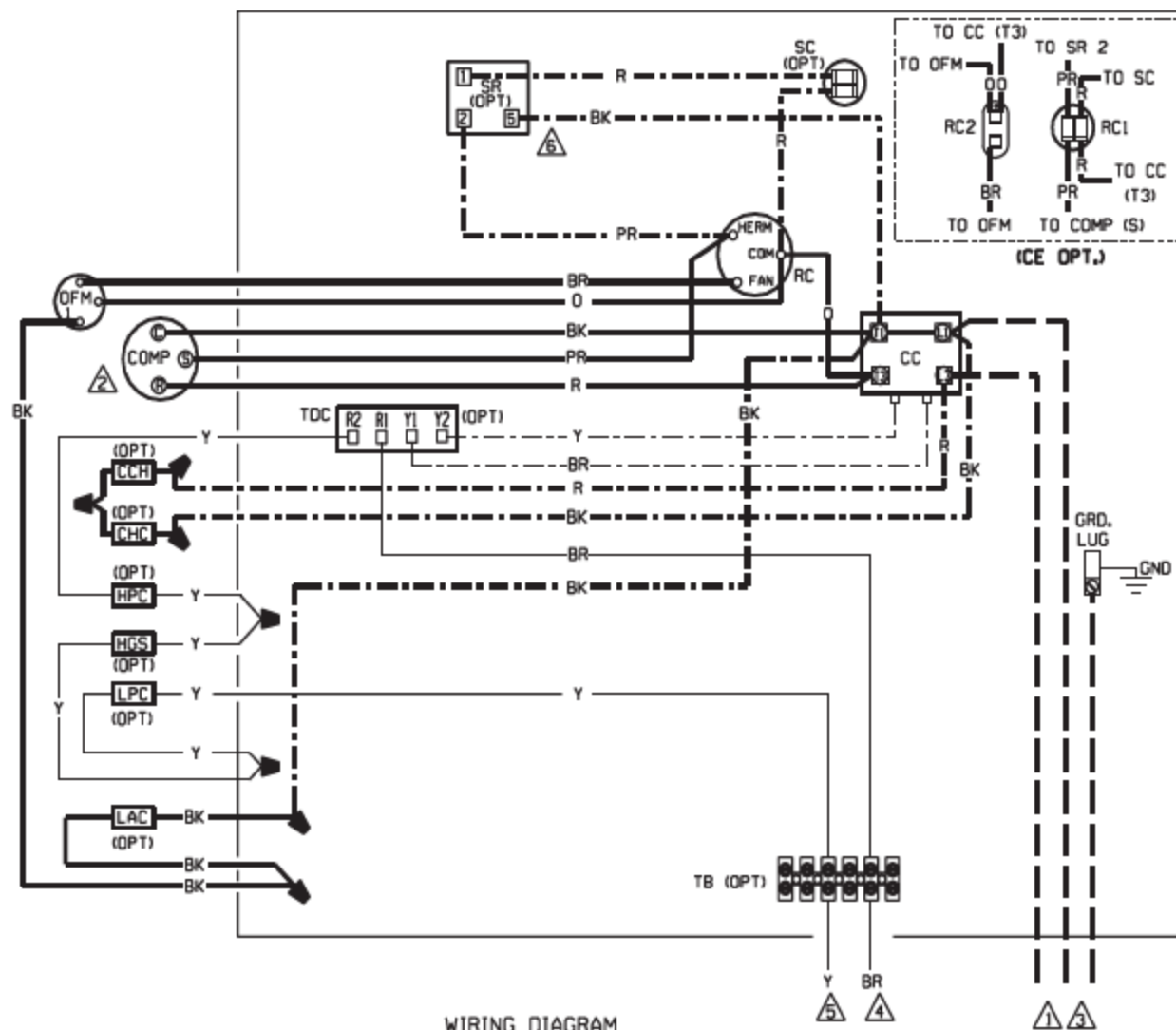
WIRING DIAGRAM
