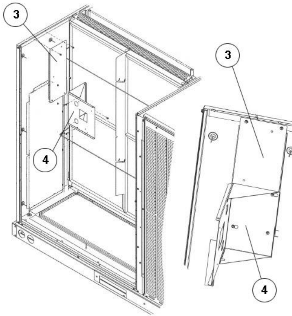
RXRX-BS03 (2) Assembly
