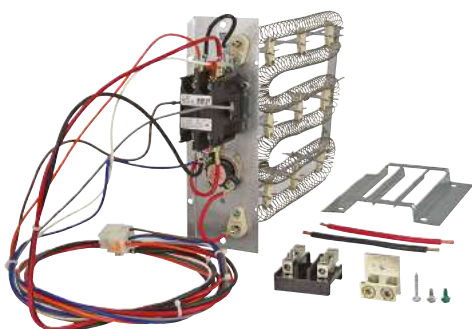
Electric Heater Kit (Sold Separately)
