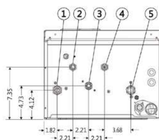
Combi Bottom (80/120)
