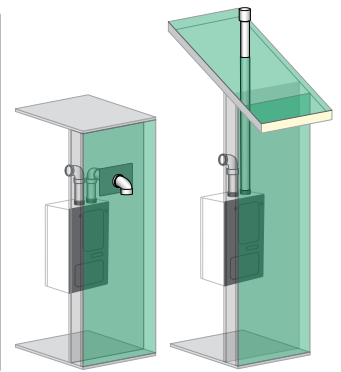
Direct exhaust
