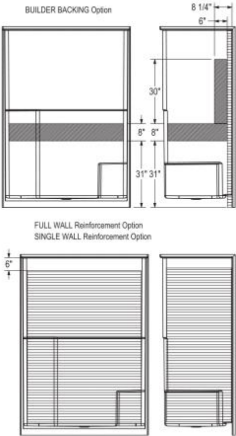
REINFORCEMENT BACKING
