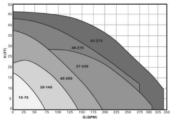
ecocirc XL High Flow Performance Range Curve
