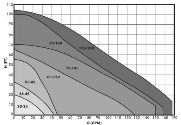
ecocirc XL High Head Performance Range Curve
