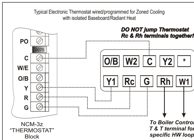
Figure 10 Electronic thermostat configured for Zone Air Cooling with separate Hot Water loop heating. Baseboard or Radiant (in floor) hot water heating loop.
