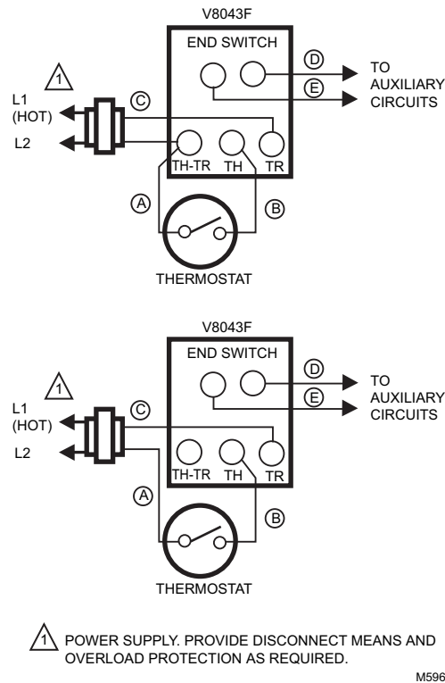
Fig. 25. Wiring a V8043F to a Taco System (2 options). (Wires are identified with letters to correspond with wires on Fig. 23.)
