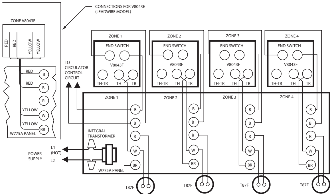
Fig. 21. Typical 4-zone system. Use an additional W775A to power up to 4 more zone valves.
