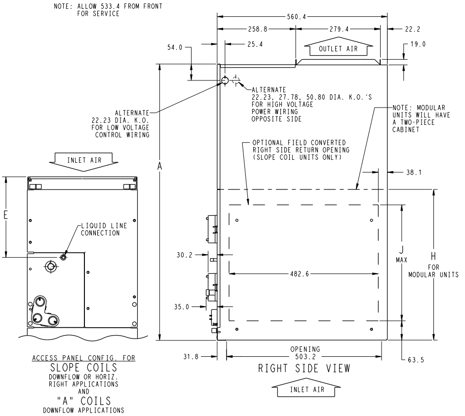
Fig. 3 – FJM - Metric (sheet 1)
