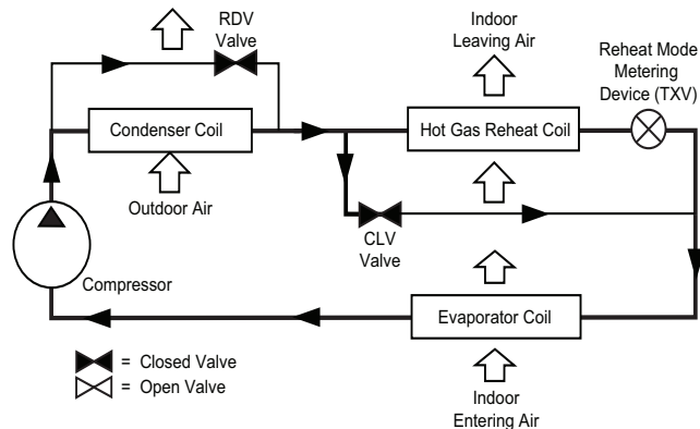
Subcooling Mode (Reheat1) — Hot Gas Re-Heat System with Single Stage Cooling
