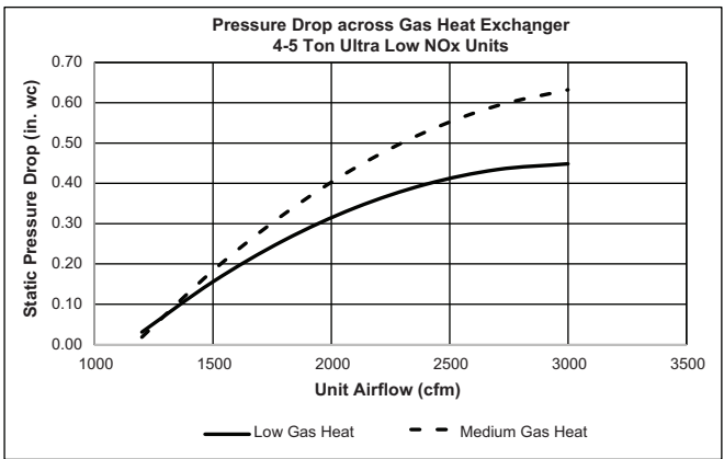
Pressure Drop across Gas Heat Exchanger, RGF Ultra Low NOx — 4 to 5 Ton Units
