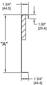
SECTION THRU SIDE
