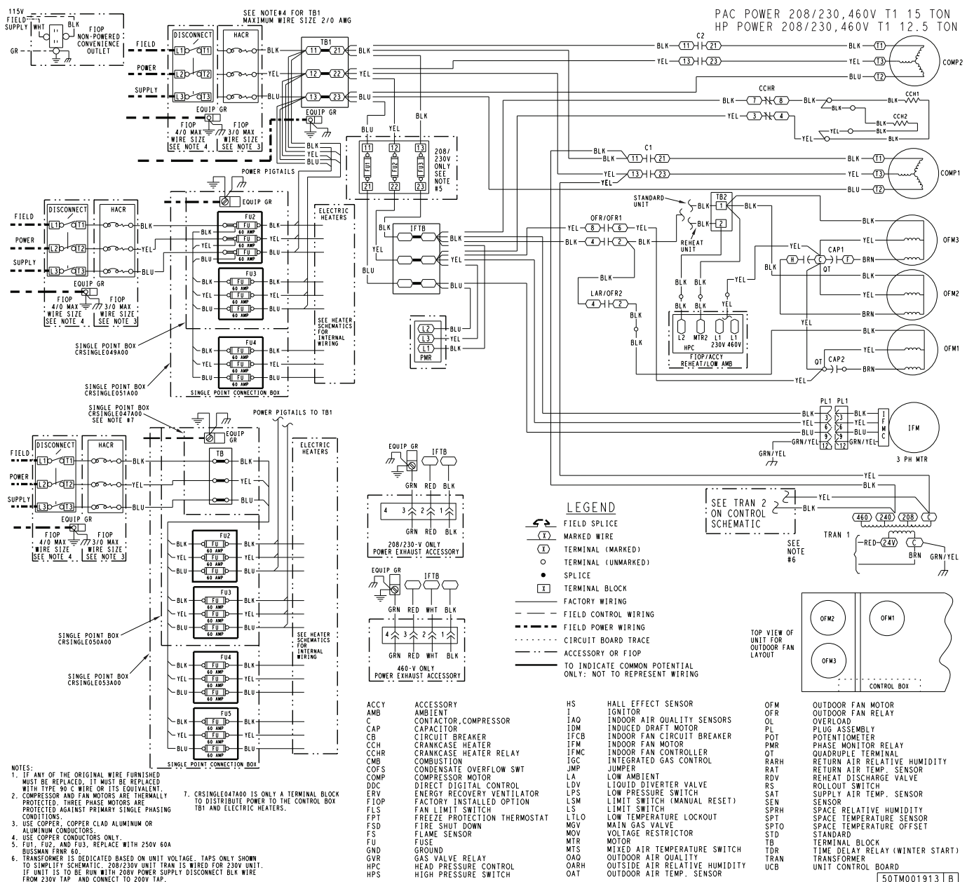
TYPICAL POWER WIRING DIAGRAM — RAV180 208-230/460-3-60 UNIT WITH ELECTROMECHANICAL CONTROLLERS
